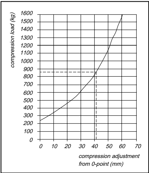
Compression load diagram
